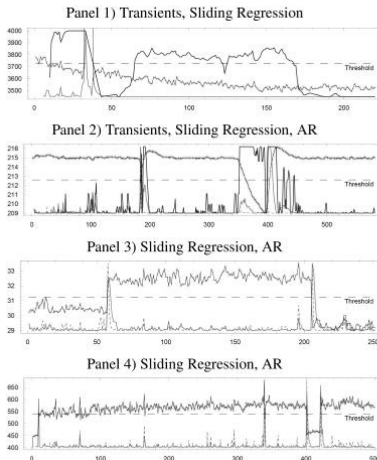
Bild 1: Examples of method performances on injection moulding data. Samples are placed along horizontal axis, vertical axis shows channel values. Instability predictions by different methods are overlaid, with 0 (no instability) at the bottom and 1 (almost certain instability) at the top of the plot. Black solid lines with + marker: channel data, dark solid lines, light grey lines, light grey dashed lines: individual detection methods.
